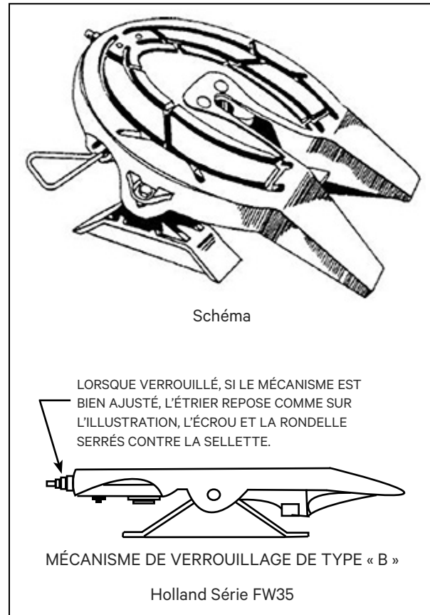
Figure 10 – Sellette
